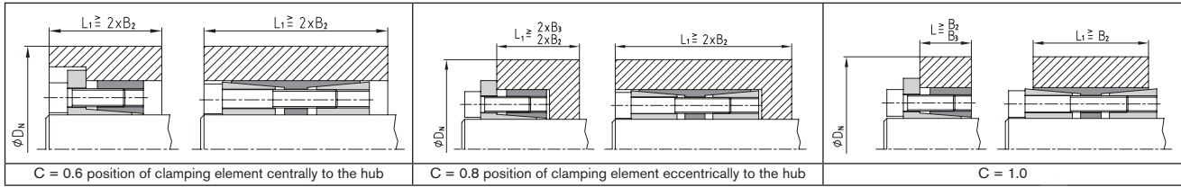
Selection table for the calculation of the external diameter of hub D_h required (correction value x )
